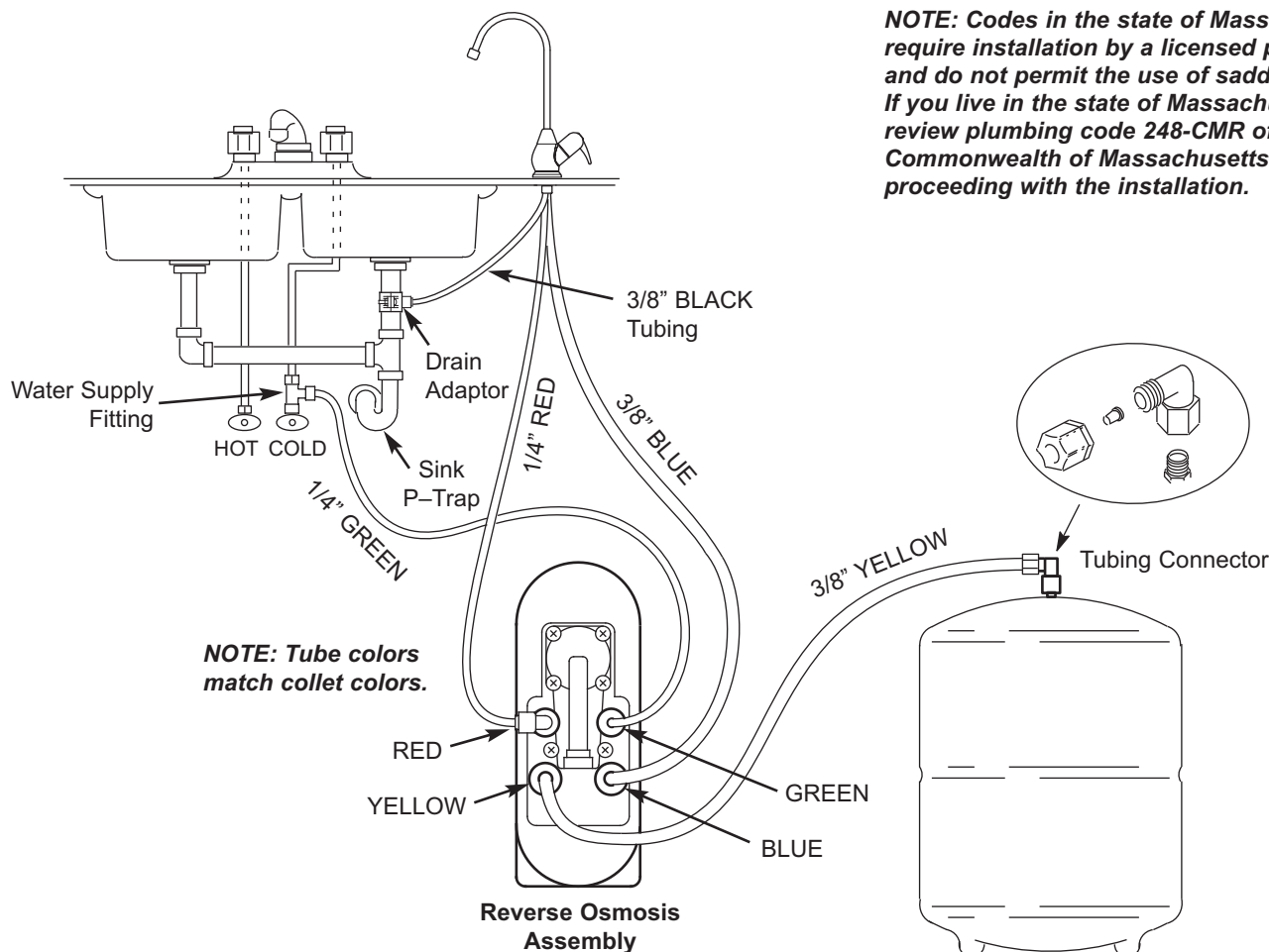
Tube Connections
